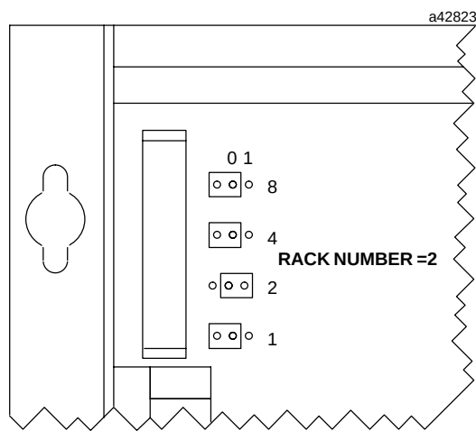
Figure 3. Rack Number Jumpers
