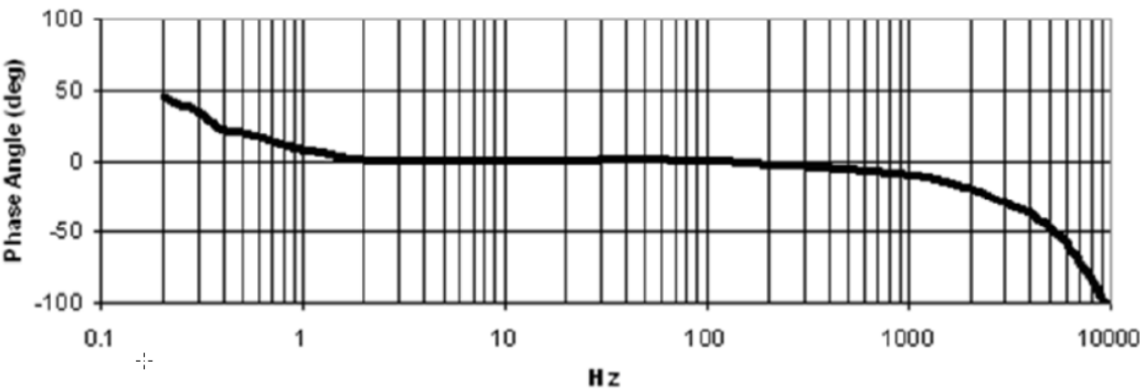
Figure 6: 200355 Accelerometer Phase
