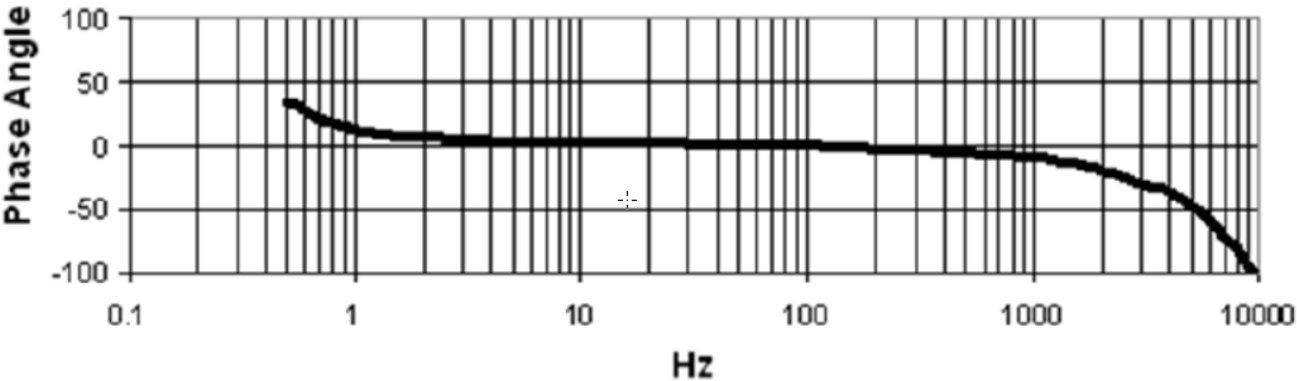
Figure 4: 200350 Accelerometer Phase
